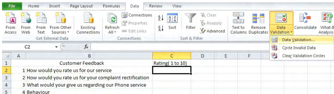
Fig. 2.11. Creating Data Validation Rule
